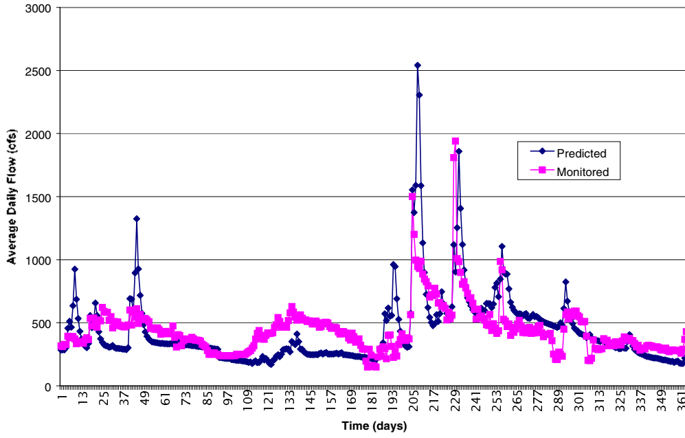
Yahara River--Gage #5430175 Predicted Vs. Measured Average Daily Flow Water Year 1999
