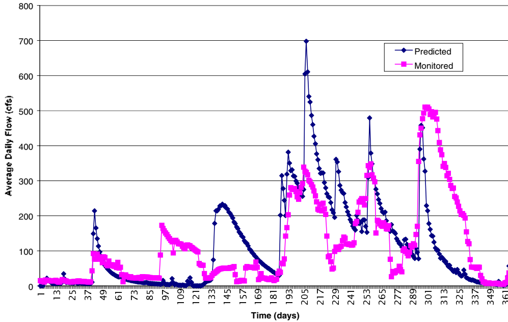
Beaver Dam River Gage #5425912 Predicted Vs. Measured Average Daily Flow Water Year 1999
