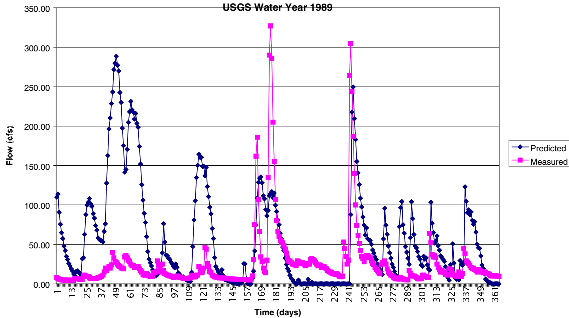
Beaver Dam River Gage #5425912 Predicted Vs. Measured Flows USGS Water Year 1989
