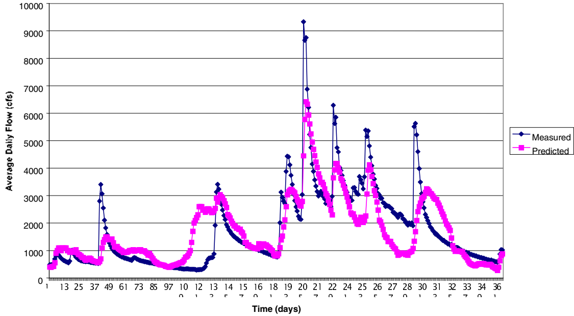
Rock River--Gage #5427080 Predicted Vs. Measured Average Daily Flow Water Year 1999
